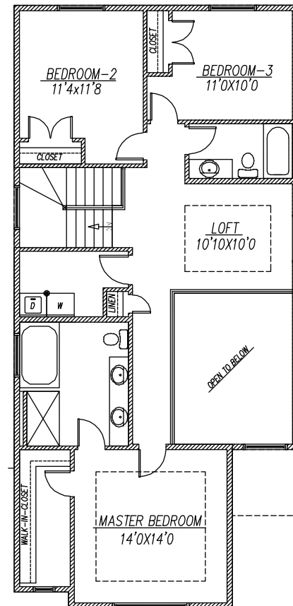
UPPER FLOOR PLAN 1111 SQ.FT.
